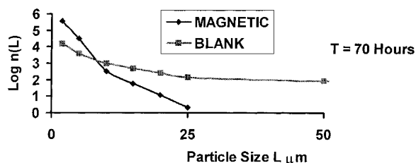
Figure 6. Effect of magnetic treatment on particle size and particle numbers over 70 hours, B = 7000 Gauss, [Ca] = 350 ppm, temperature = 60°C.
