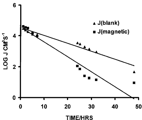
Figure 7. Change in nucleation rate brought about by magnetic treatment. B = 7000 Gauss, [Ca] = 350 ppm, temperature = 60^\circ\text{C} .
