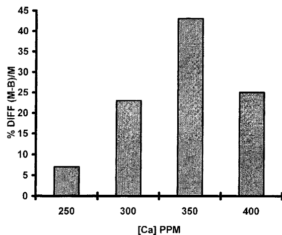
Figure 3. Effect of calcium carbonate concentration on the magnetically-induced change in reaction rate constant, B = 7000 Gauss, temperature = 55°C.
