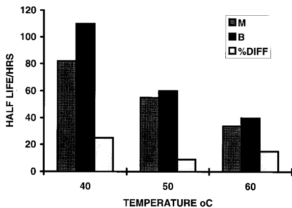
Figure 2. Effect of temperature on the reaction half life for the formation of calcium carbonate.
