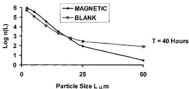
Figure 4. Reproducibility of magnetically-enhanced scale amelioration, B = 7000 Gauss, temperature = 60°C, [Ca] = 350 ppm.
