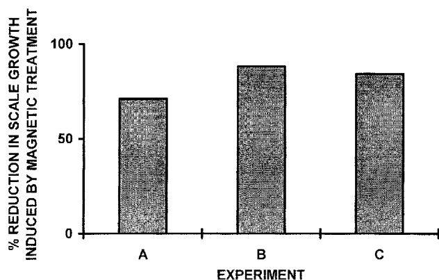
Figure 4. Reproducibility of magnetically-enhanced scale amelioration, B = 7000 Gauss, temperature = 60°C, [Ca] = 350 ppm.
