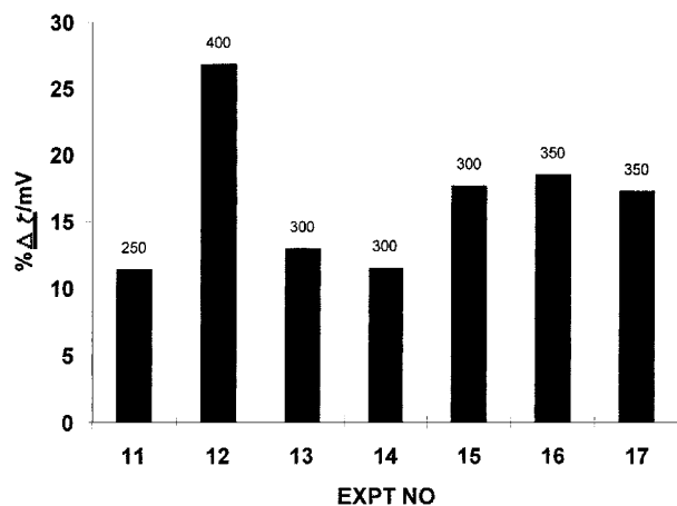
Figure 5. Percentage reduction in zeta potential after magnetic treatment for a range of calcium concentrations. B = 7000 Gauss, temperature = 60°C. Concentrations shown are all in ppm.
