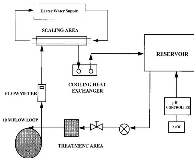
Figure 1. Flow diagram of experimental test rig.
